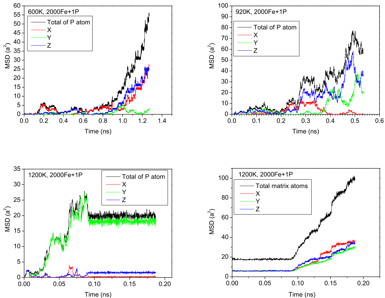
FIG. 3: Mean Squared Displacement (MSD) against time for migration in a unit cell containing 2000 Fe and 1P atom, initially located in a mixed dumbbell. Various temperatures were examined: at 600K and 920K the P remains attached to the interstitial throughout the period of the run. For 1200K, we observed rapid 1D diffusion of the phosphorus atom via mixed interstitial (Fe does not diffuse in this phase), followed by a dissociation event and standard interstitial diffusion in pure Fe. The simulation box is large enough that the interstitial is not recaptured, and subsequent diffusion is for the iron atoms.
