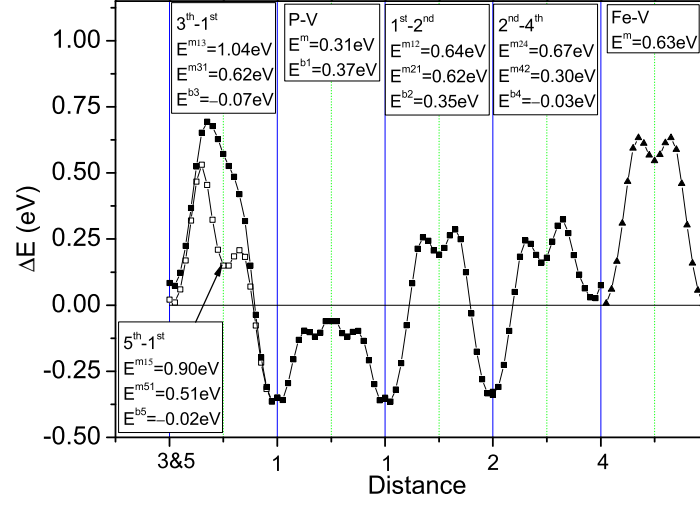
FIG. 2: Constrained static relaxations of P-vacancy complex with P moved over various barriers. E^{mxy} gives the height of the barrier for the P to move from x^{th} neighbour to the y^{th} , E^{bx} gives the binding energy of P at the x^{th} neighbour site. The final panel shows the barrier for vacancy movement in pure iron. The barrier against motion of the vacancy-phosphorus complex is similar to the binding energy, and much lower than the barrier in pure Fe. Consequently, the P traps the vacancy, reducing overall vacancy diffusion.
