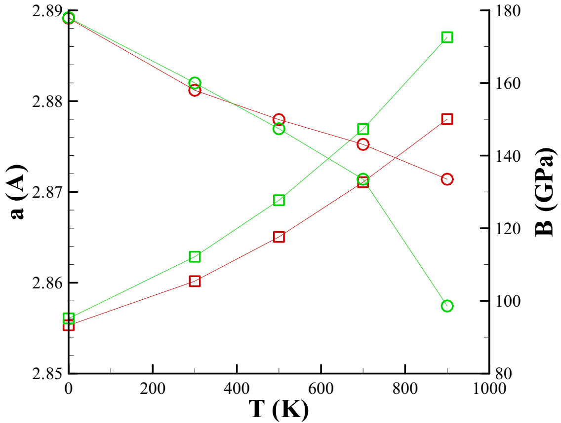
Lattice parameters (squares) and bulk moduli (circles) for Fe (1000 atoms, red lines) and Fe 90 P 10 (2000 atoms, green line).
